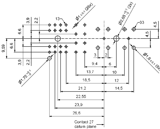
PCB-hole pattern (34 positions)
