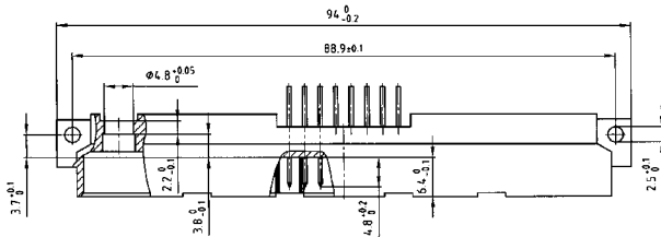
Solder pin angled T
