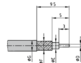
Wire stripping
