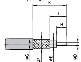
Wire stripping
