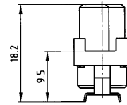
Female connector with strain relief
