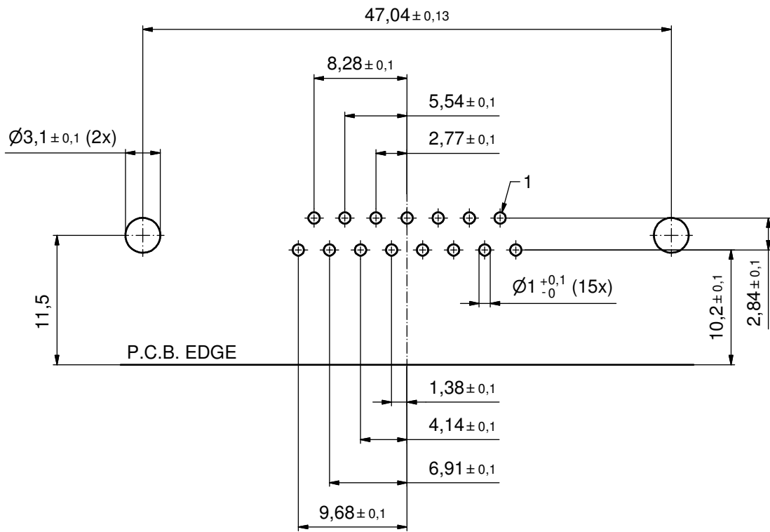
P.C.B. HOLE DRILLINGS (P.C.B. TOP SIDE)
